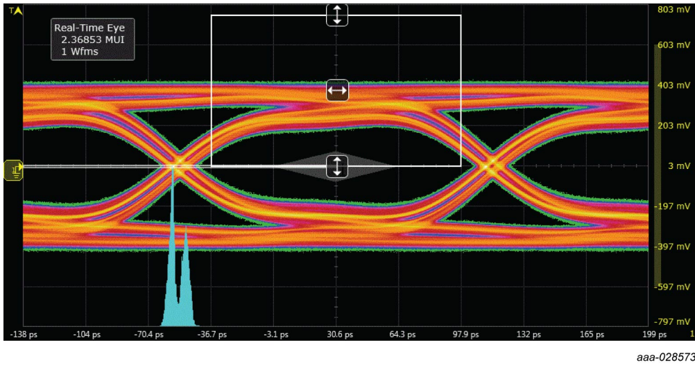
Figure 9. HDMI 2.0 eye diagram TP1, test board with PESD3USB3B/C; typical values
