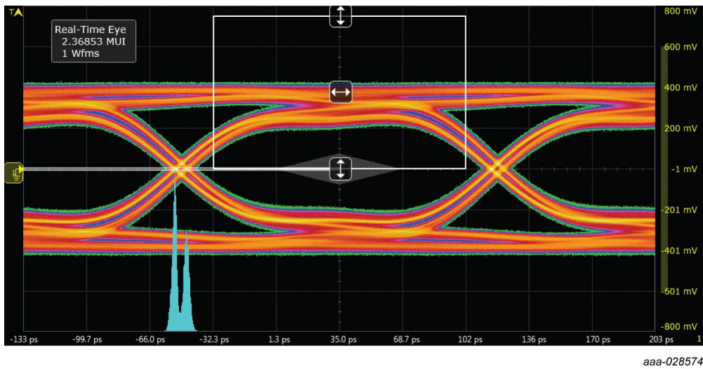
Figure 10. HDMI 2.0 eye diagram TP1, test board without device; typical values
