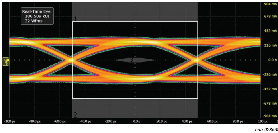
Figure 5. USB3.2 eye diagram 10 Gbps, test board with PESD3USB3B/C; typical values
