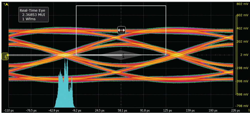
Figure 11. HDMI 2.0 eye diagram TP2, test board with PESD3USB3B/C; typical values
