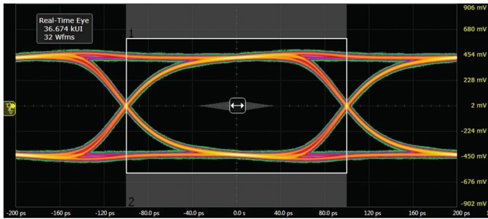
Figure 7. USB3.2 eye diagram 5 Gbps, test board with PESD3USB3B/C; typical values
