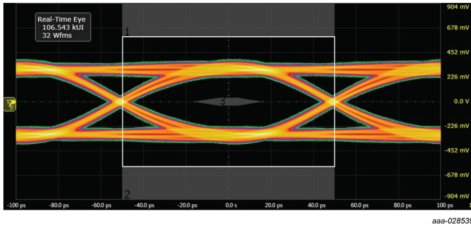
Figure 6. USB3.2 eye diagram 10 Gbps, test board without device; typical values
